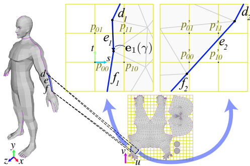
Fig. 3. A seam edge e on the 3D surface mesh corresponds to two half-edges e_1 and e_2 in the u, v parameterization. Similarly, for other edges d, f . We use boldface \mathbf{e}_i(\gamma) to refer to the vector-valued function mapping a relative 1D position along on the edge to its half-edge positions along e_1 in u, v space. The half-edges e_1 and e_2 will pass through (possibly different) texels where signals stored at corners ( p_{00}, p_{01} , etc.) are bilinearly interpolated.
